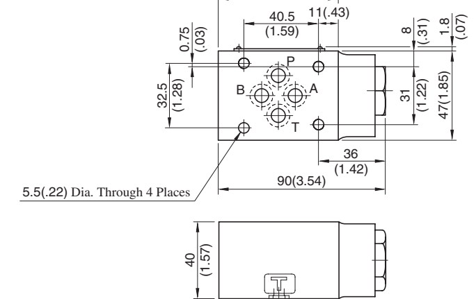
MCP-01 MCT-01
